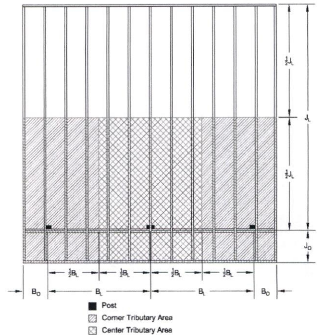
Figure B1. Examples of Tributary Areas
