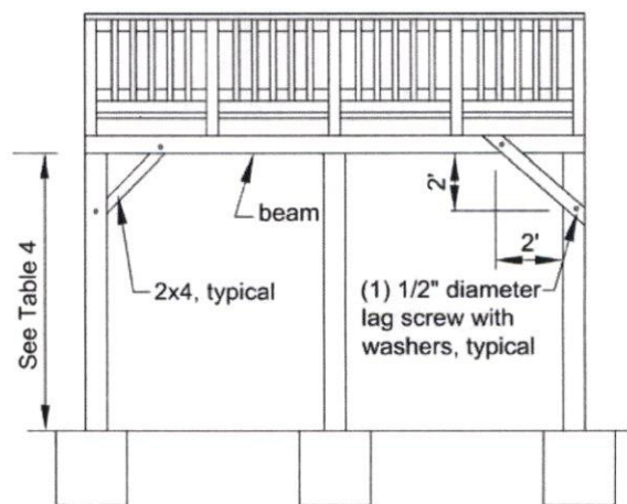
Figure 10. Diagonal Bracing.
